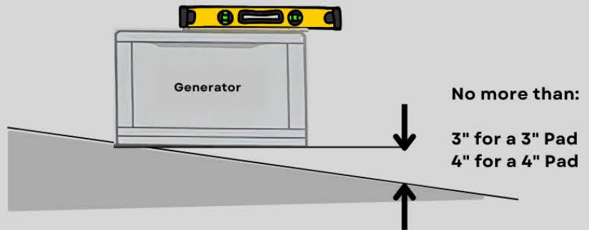
Genpads must be set on a close to level surface. There can be no more than 3" difference in height across the length of a 3" thick Genpad, or 4" difference for a 4" thick Genpad.
